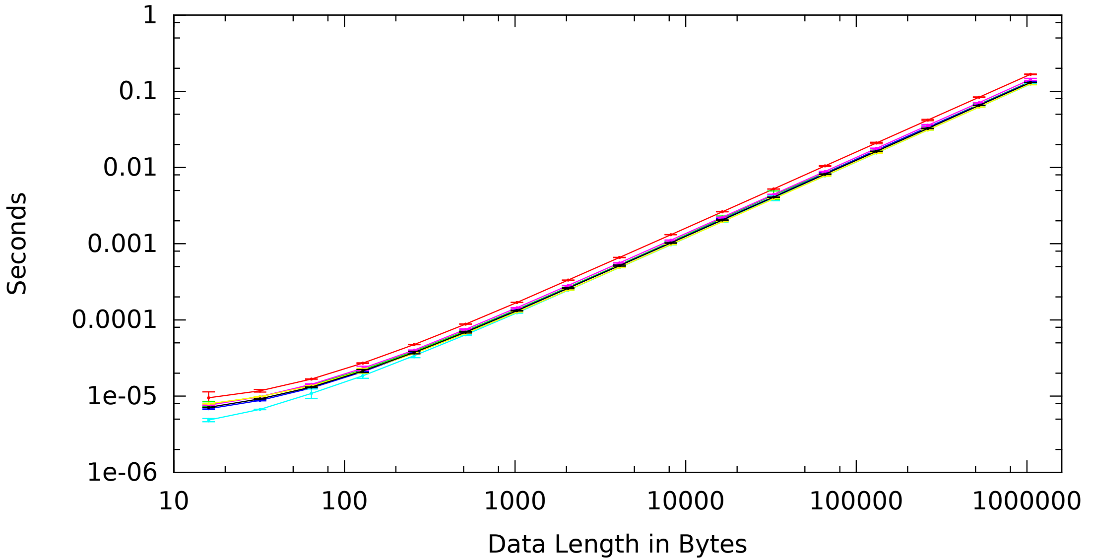
atom-1600-debian-wheezy Rijndael: Absolute Time by Data Length
