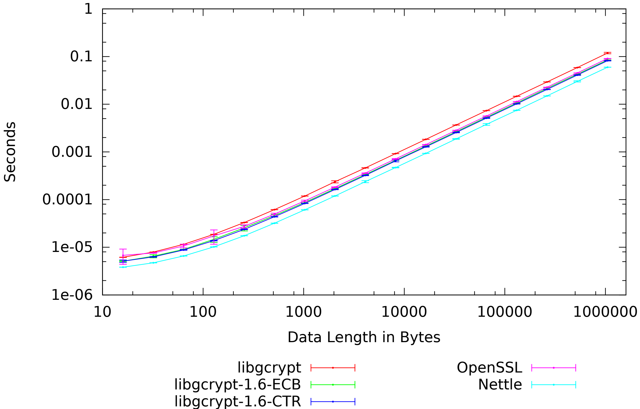
atom-1600-debian-wheezy CAST5: Absolute Time by Data Length
