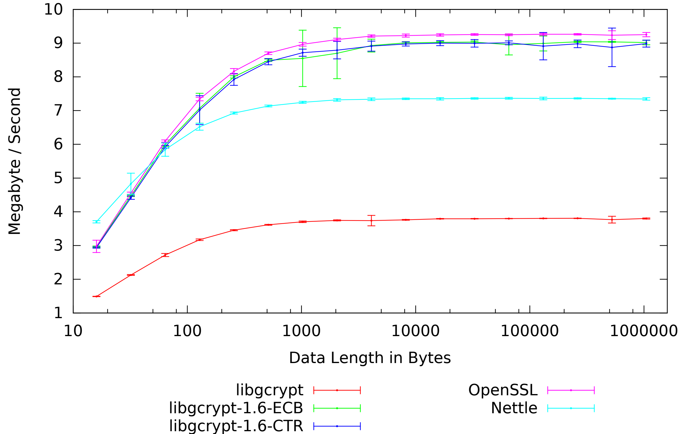
atom-1600-debian-wheezy Camellia: Speed by Data Length
