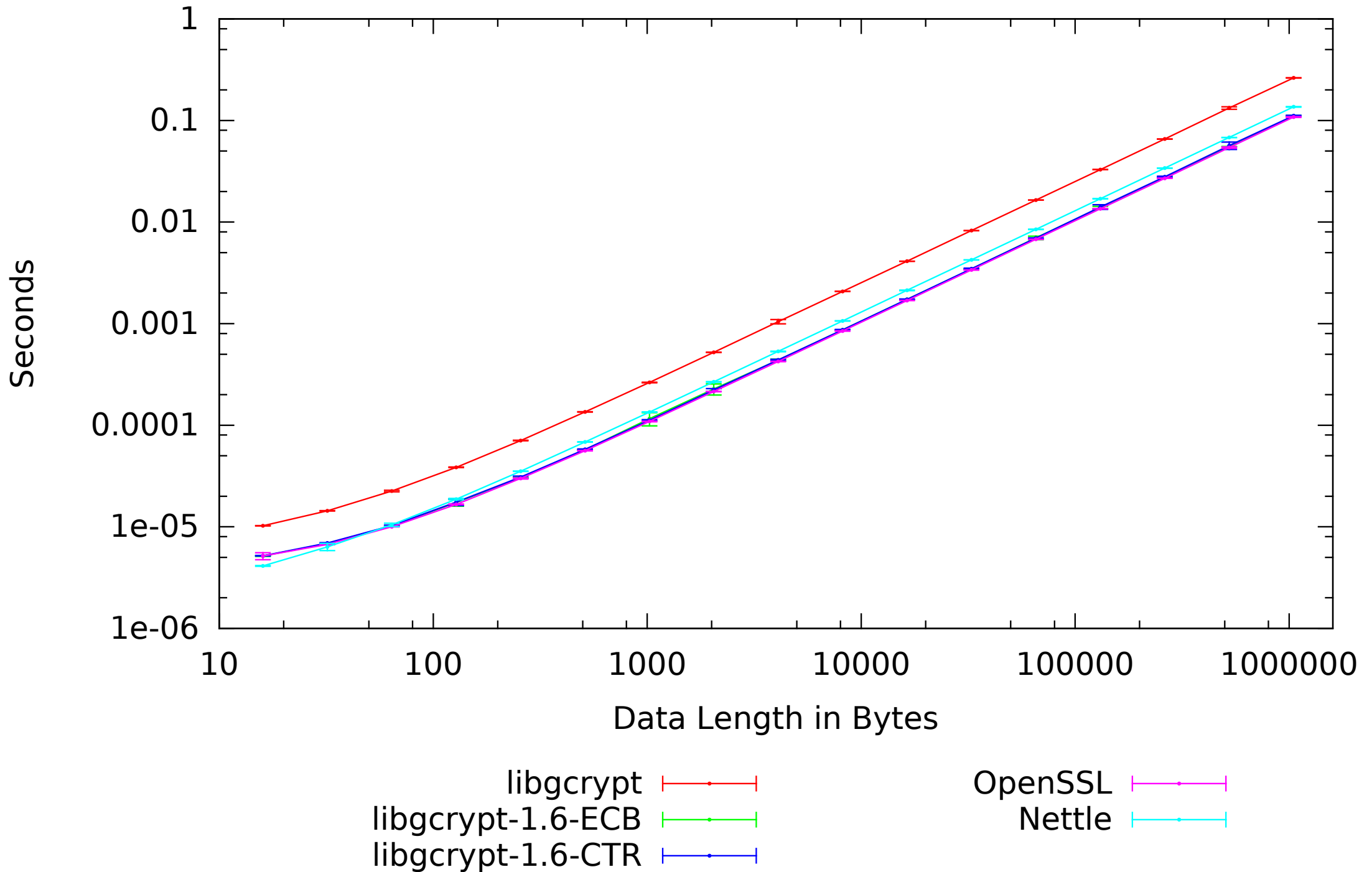
atom-1600-debian-wheezyCamellia: Absolute Time by Data Length
