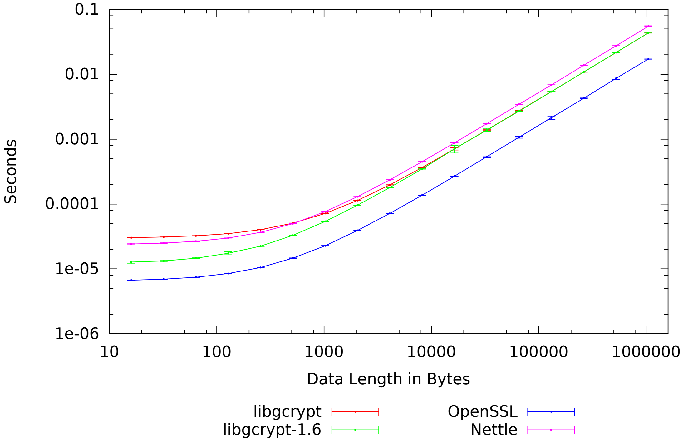
atom-1600-debian-wheezy ARC4: Absolute Time by Data Length
