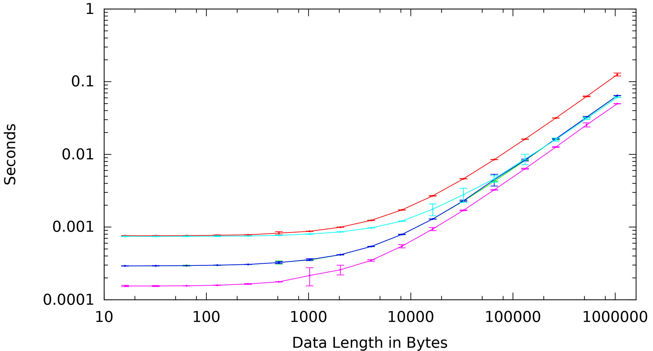
atom-1600-debian-wheezy Blowfish: Absolute Time by Data Length
