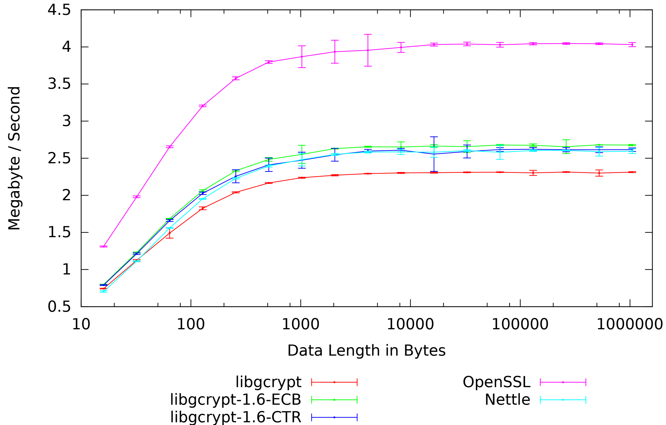
atom-1600-debian-wheezy Triple DES: Speed by Data Length
