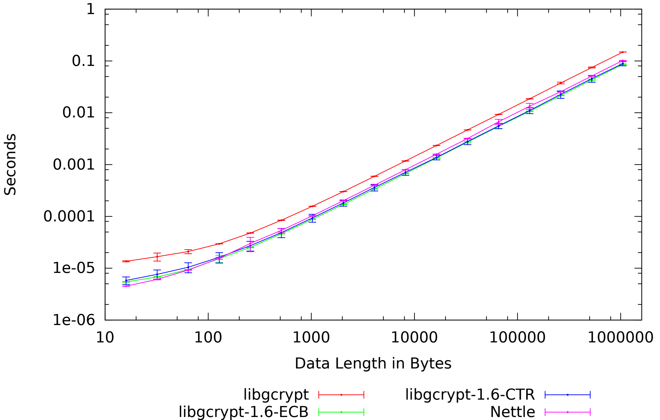
atom-1600-debian-wheezy Serpent: Absolute Time by Data Length
