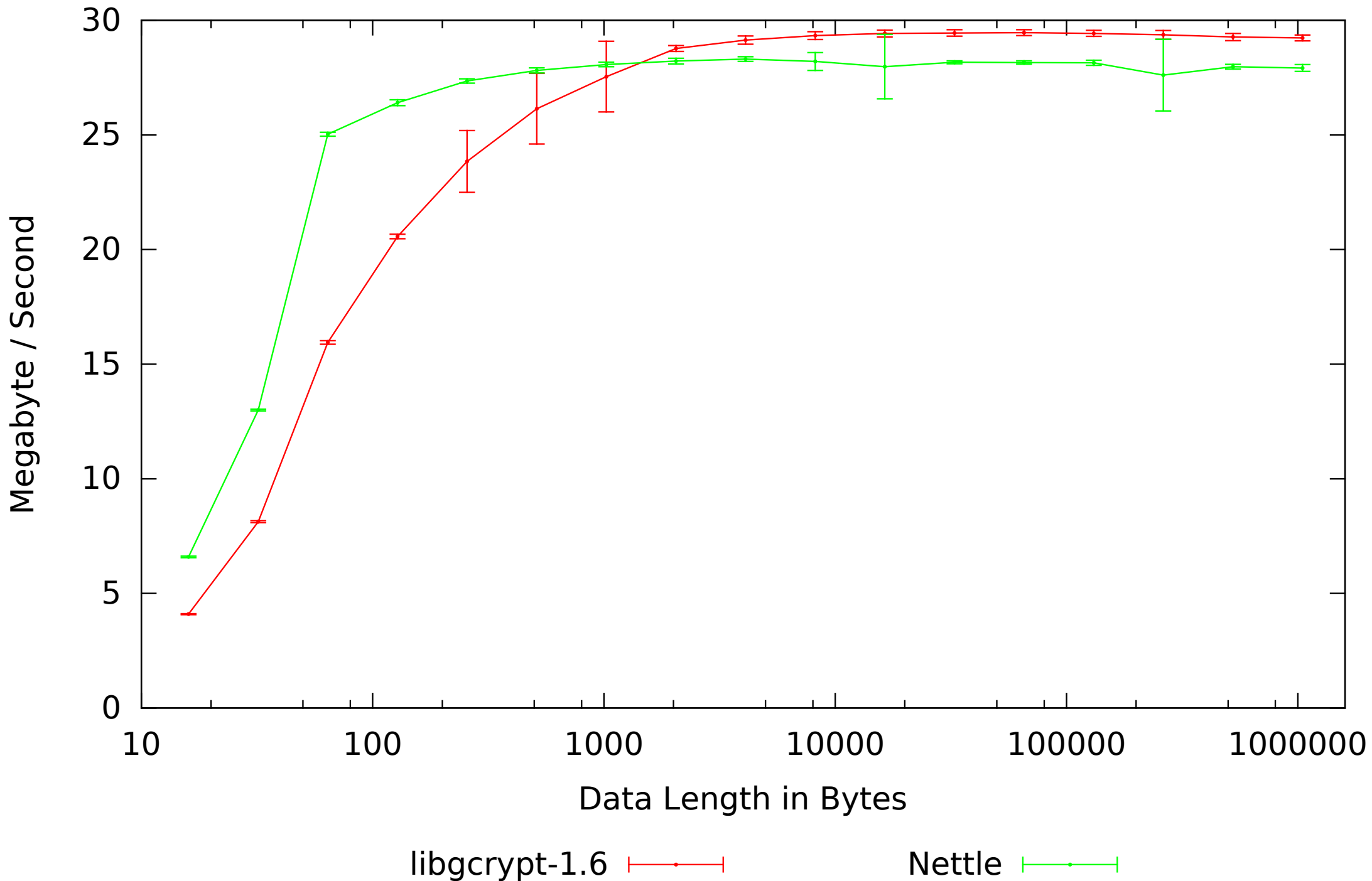
atom-1600-debian-wheezy Salsa20: Speed by Data Length
