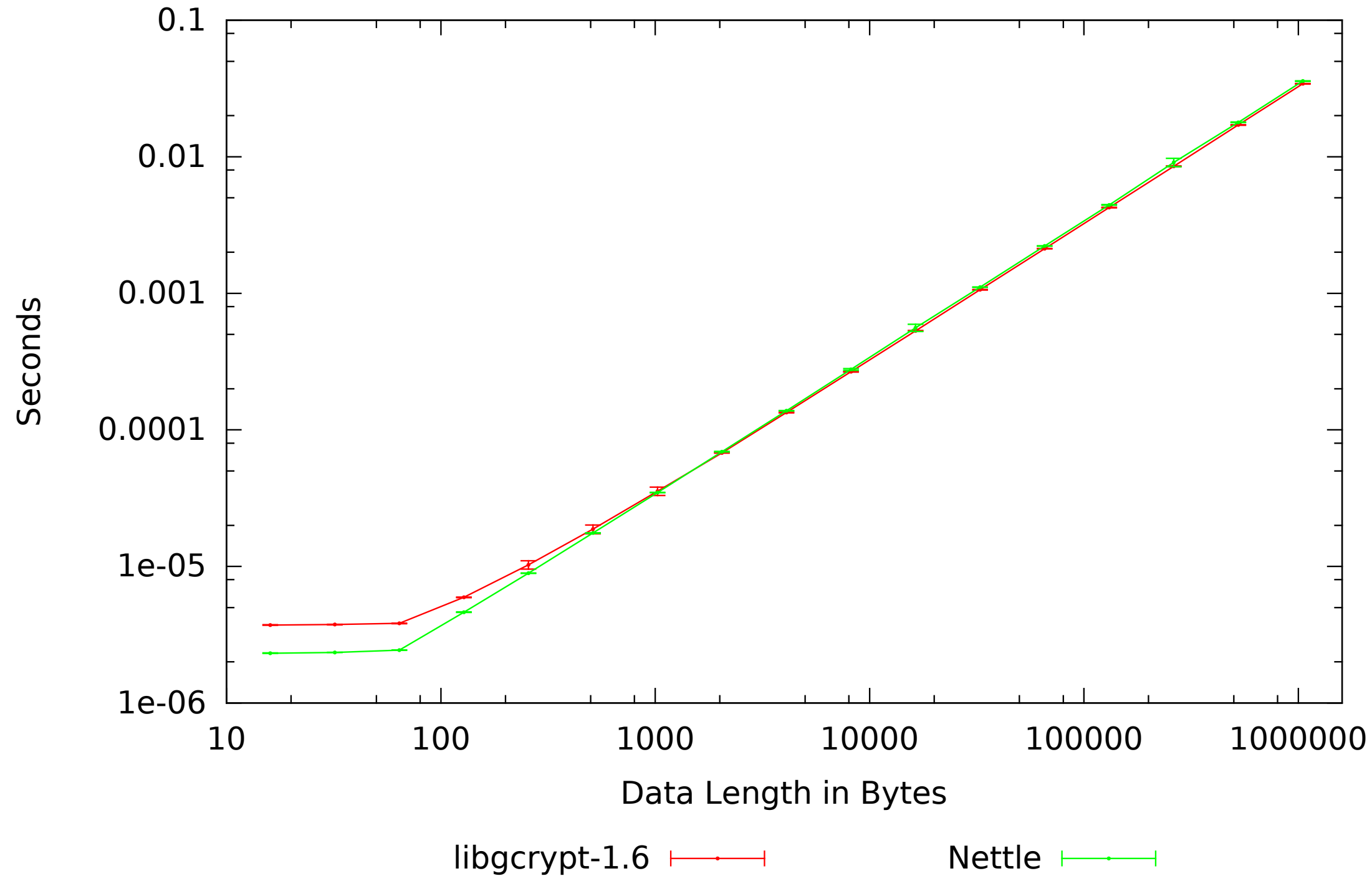
atom-1600-debian-wheezy Salsa20: Absolute Time by Data Length
