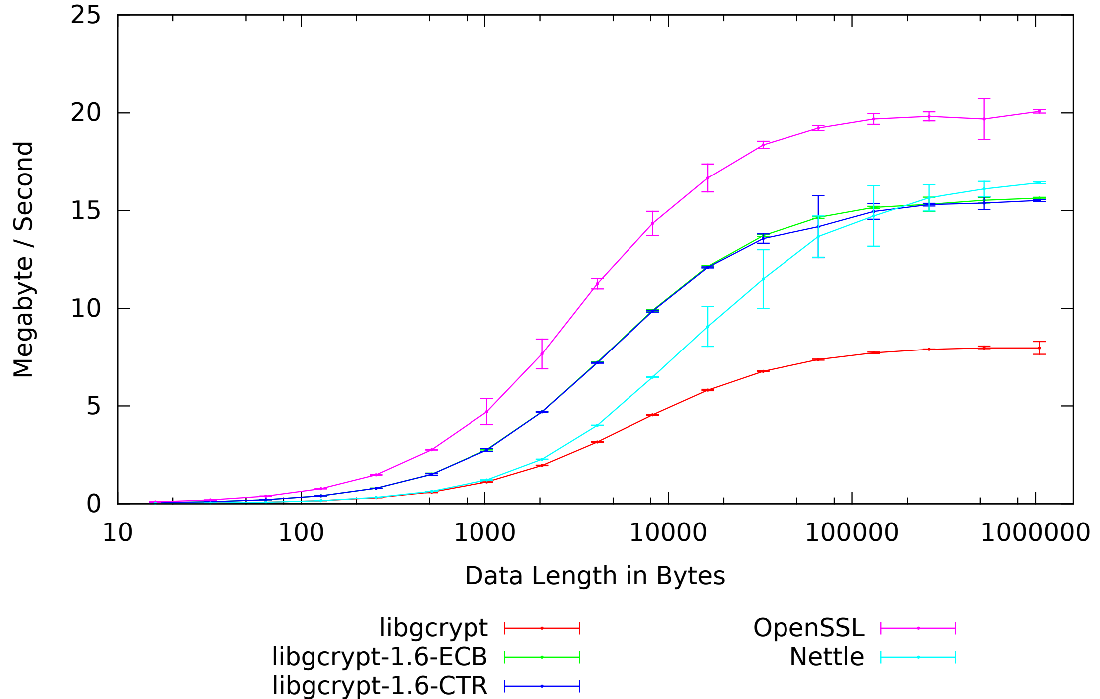
atom-1600-debian-wheezy Blowfish: Speed by Data Length
