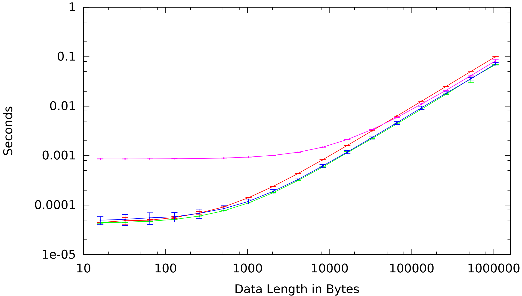
atom-1600-debian-wheezy Twofish: Absolute Time by Data Length
