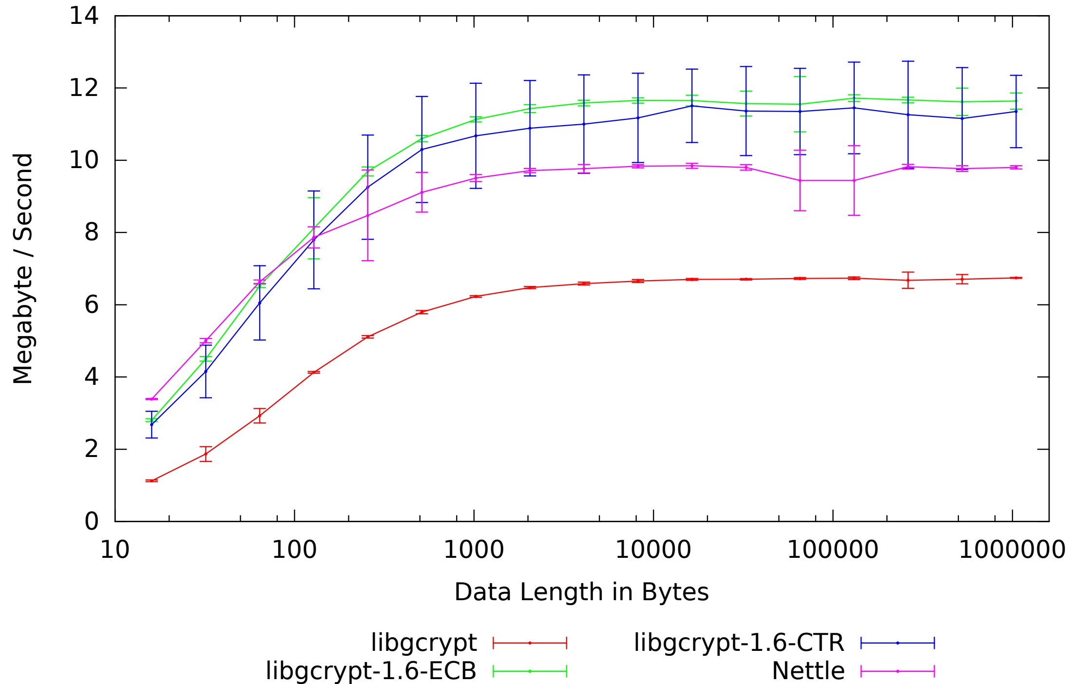
atom-1600-debian-wheezy Serpent: Speed by Data Length
