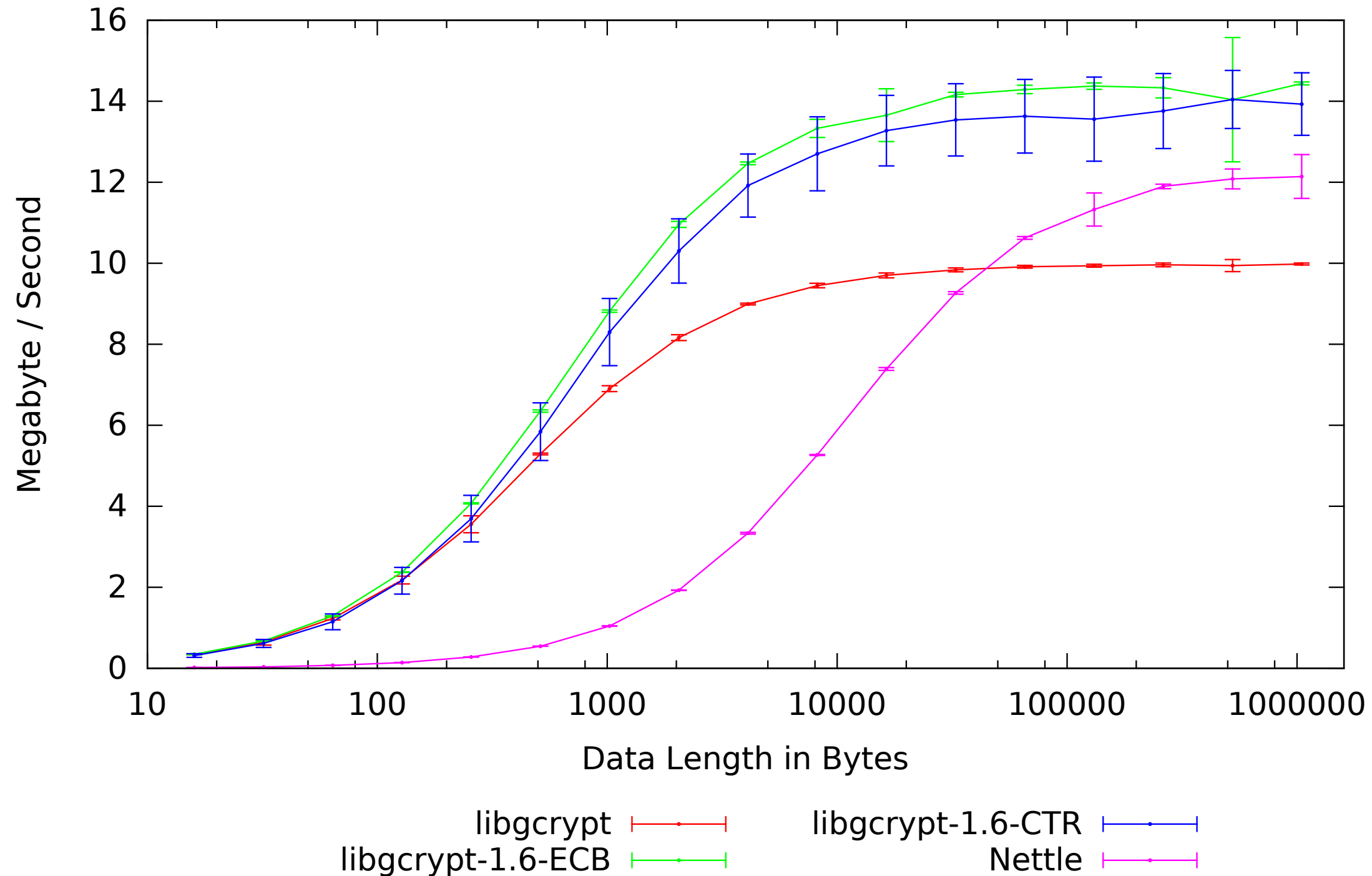
atom-1600-debian-wheezy Twofish: Speed by Data Length
