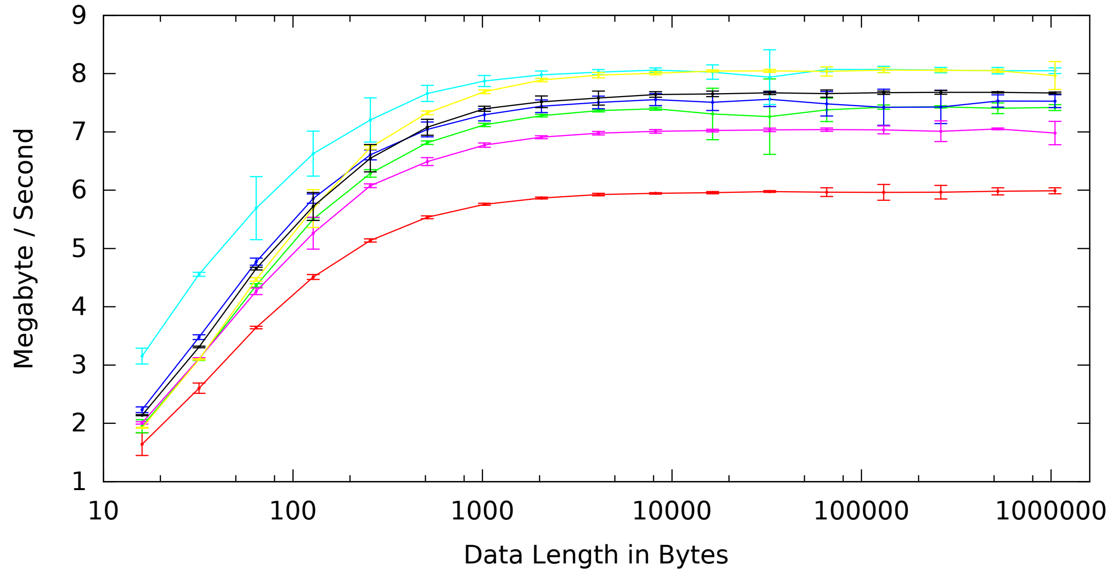
atom-1600-debian-wheezyRijndael AES: Speed by Data Length
